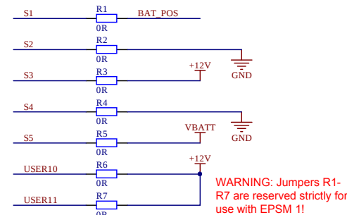
Power Connection Jumpers
