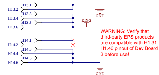
EPSM1 Ring Bus Connection
