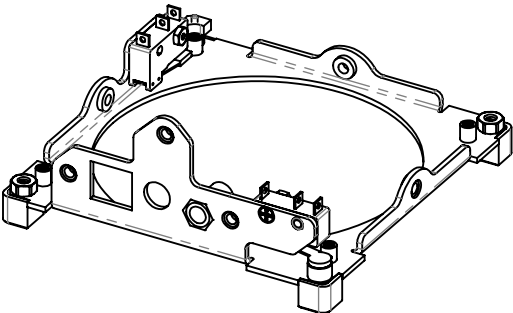
710-02203 BASE PLATE, LARGE APERTURE, DUAL SWITCH
