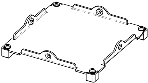
710-00295 COVER PLATE, SOLID
