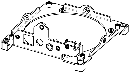
710-00783 BASE PLATE, ANTS, SINGLE SWITCH
