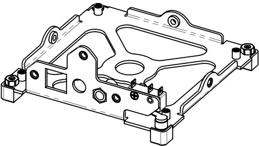
710-00294 BASE PLATE, SKELETON, SINGLE SWITCH
