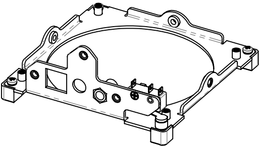
710-02302 BASE PLATE, LARGE APERTURE, SINGLE SWITCH
