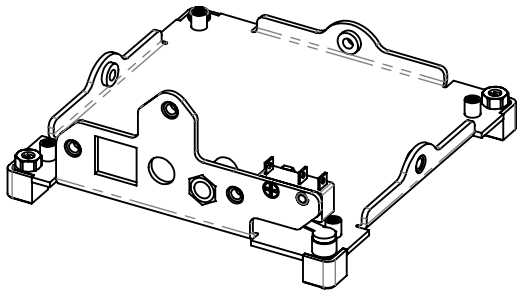
710-00293 BASE PLATE, SOLID, SINGLE SWITCH
