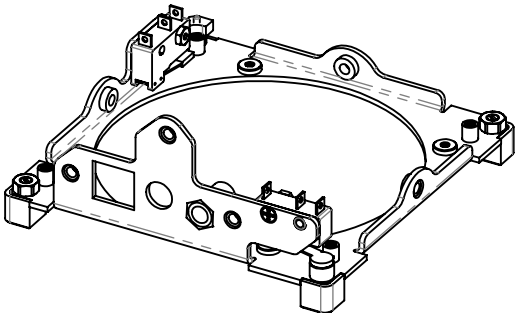
710-00960 BASE PLATE, ANTS, DUAL SWITCH
