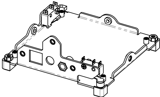
710-00793 BASE PLATE, SOLI, DUAL SWITCH
