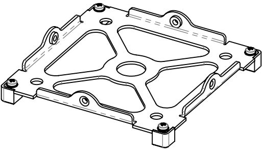
710-00296 COVER PLATE, SKELETON
