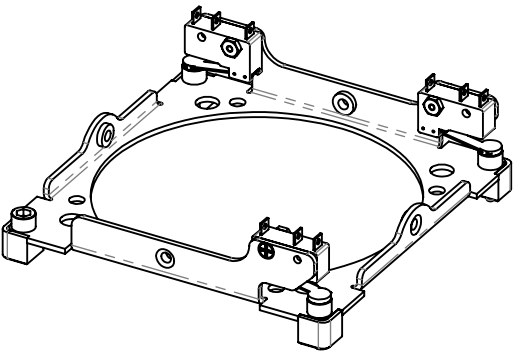
711-01873 COVER PLATE, LARGE APERTURE TRI SWITCH
