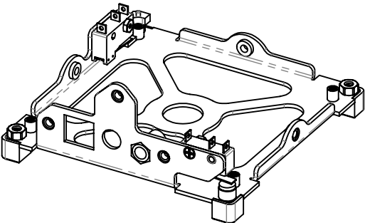
710-00794 BASE PLATE, SKELETON, DUAL SWITCH
