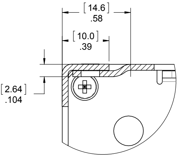
DETAIL C SCALE 2 : 1
